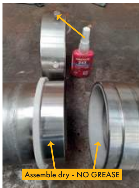
Swivel joint. Remove M8 bolts to disassemble. Do NOT assemble with grease. Assemble dry only. Strip and clean regularly
